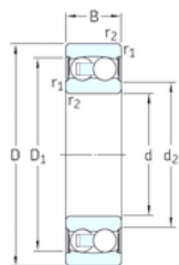
Cylindrical bore
